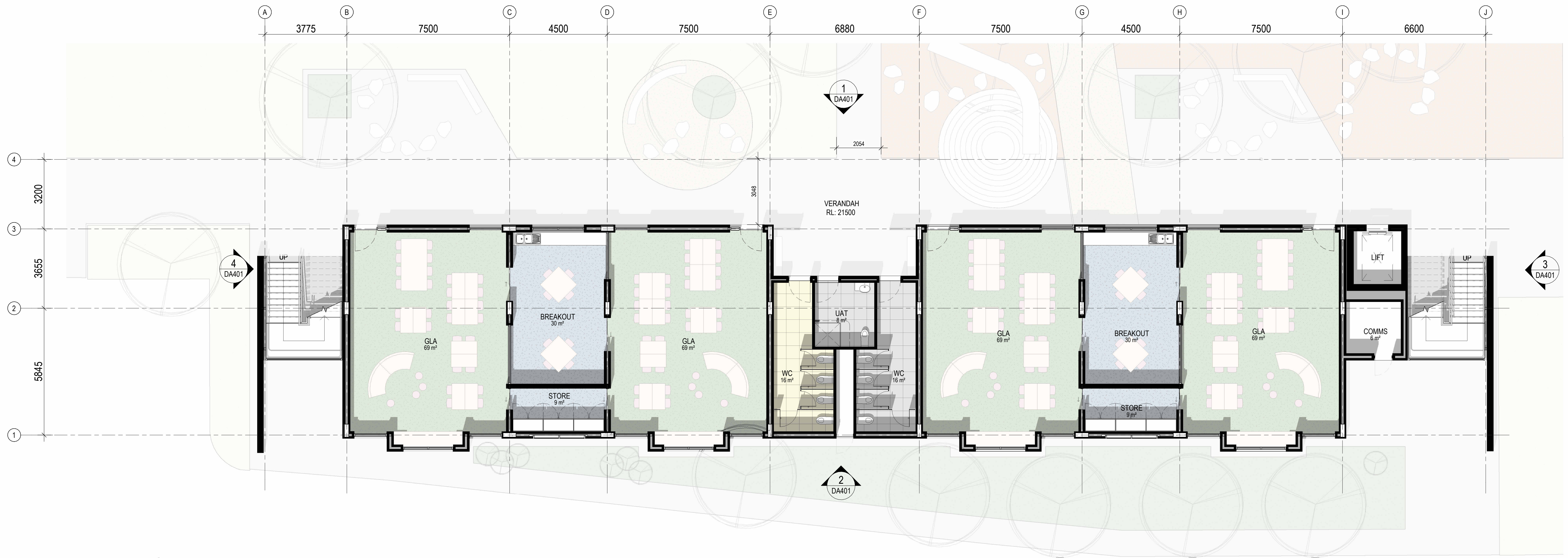
1 FLOOR PLAN - GLA BLOCK GROUND 1:100
