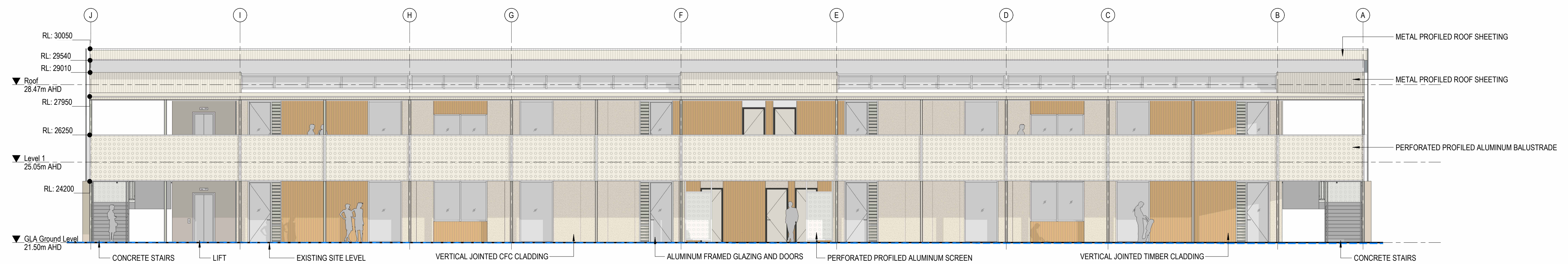
1 GLA BLOCK - ELEVATION 1:100
