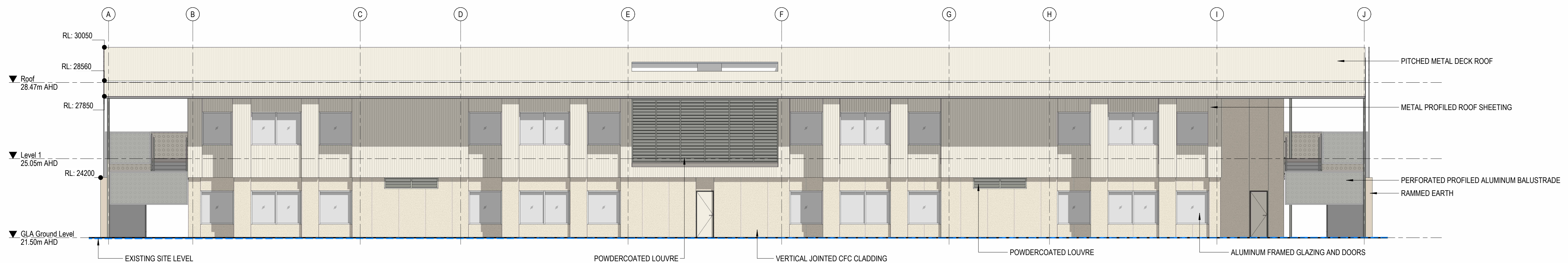
2 GLA BLOCK - ELEVATION 1:100
