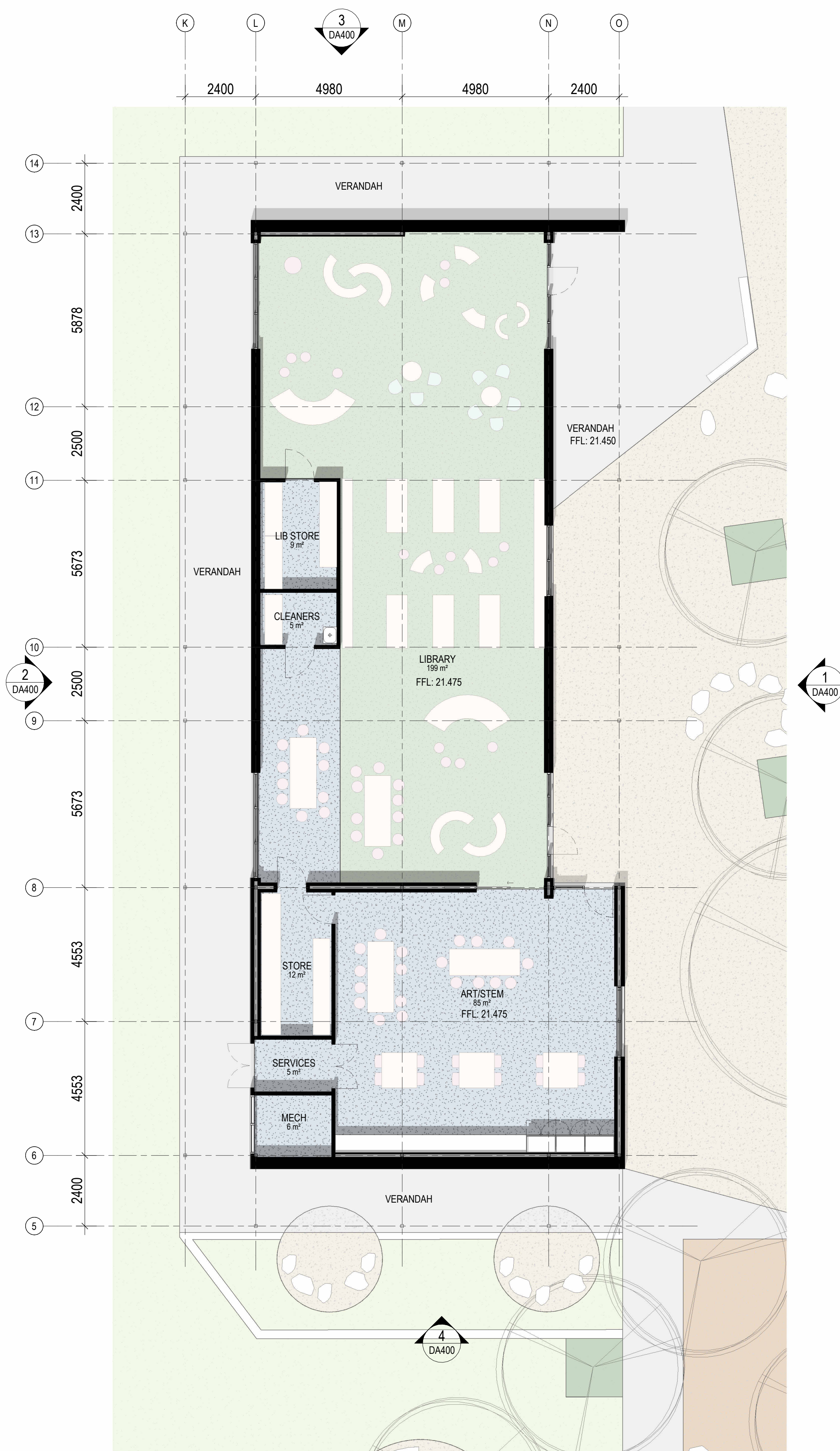
1 PROPOSED NEW LIBRARY - FLOOR PLAN 1:100
