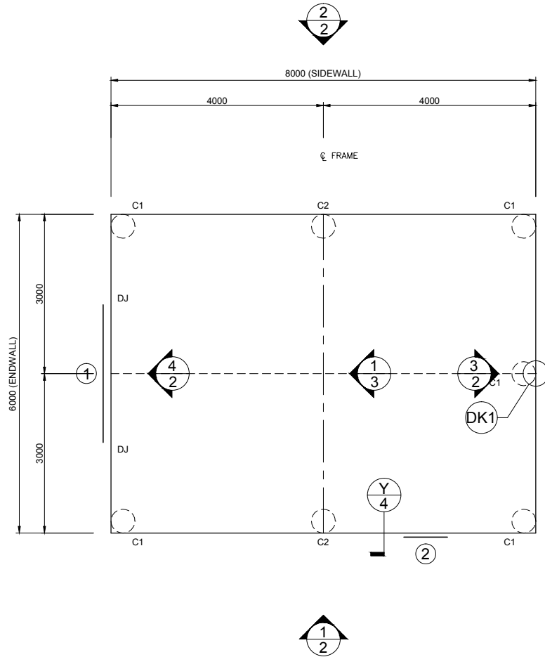
1 FOUNDATION PLAN AND MEMBER LAYOUT SCALE: 1 = 100
