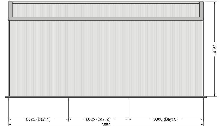
South elevation
