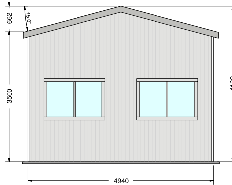
West elevation
