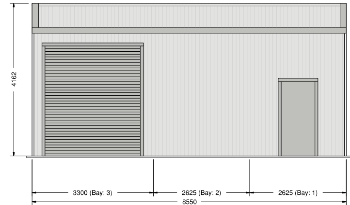
North elevation
