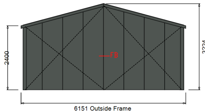
Front External Elevation
