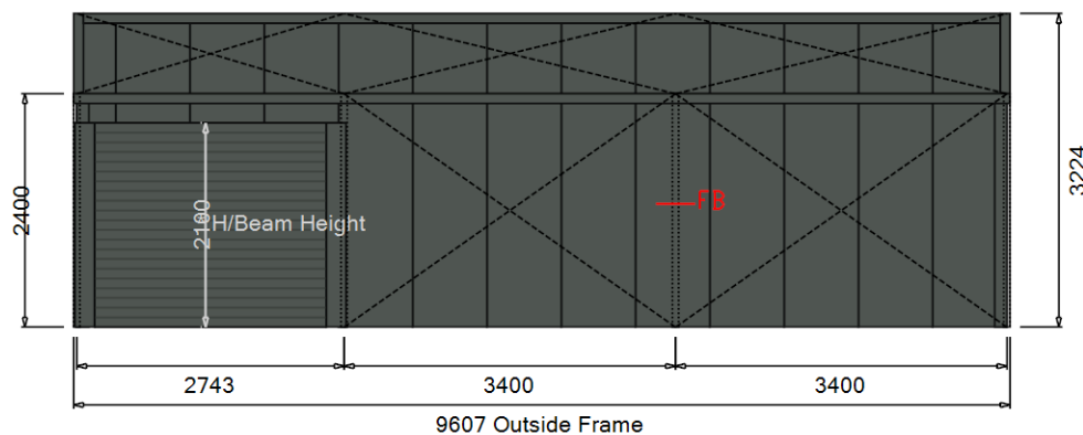
Left Elevation
