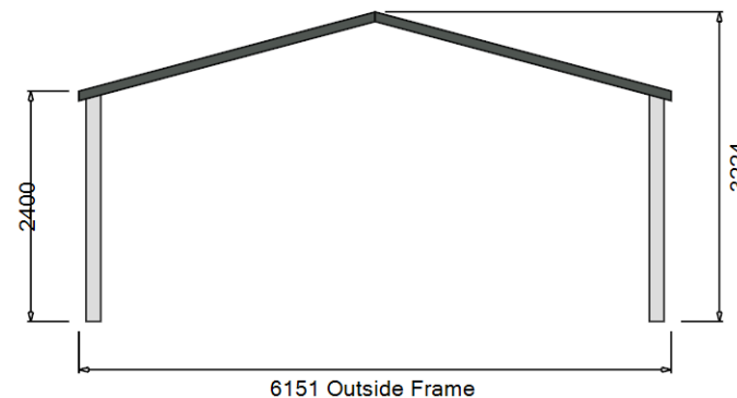
Rear Internal Elevation - 2
