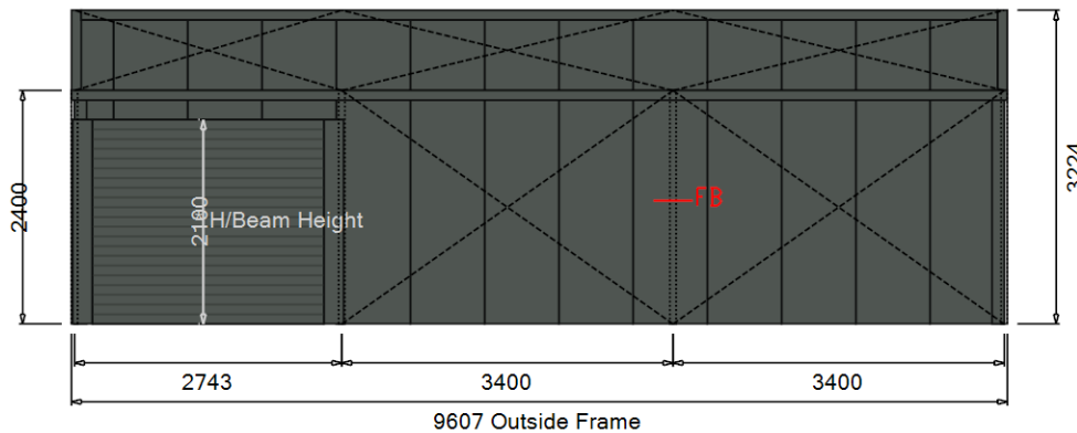
Left Elevation
