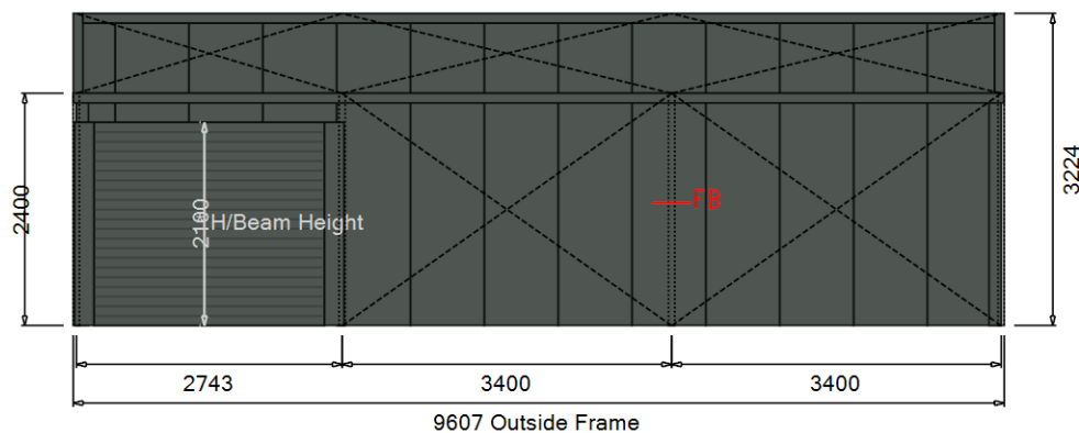
Left Elevation
