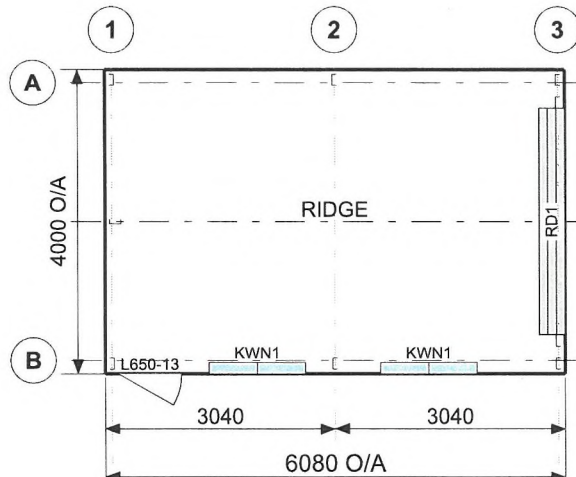
FRAME ROOF PLAN
